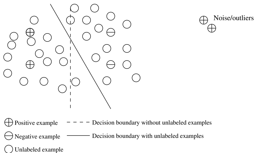
Figure 1.12 Semi-supervised learning.
