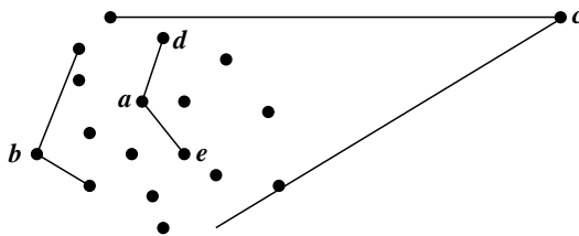
Figure 12.15 Angle-based outliers.
