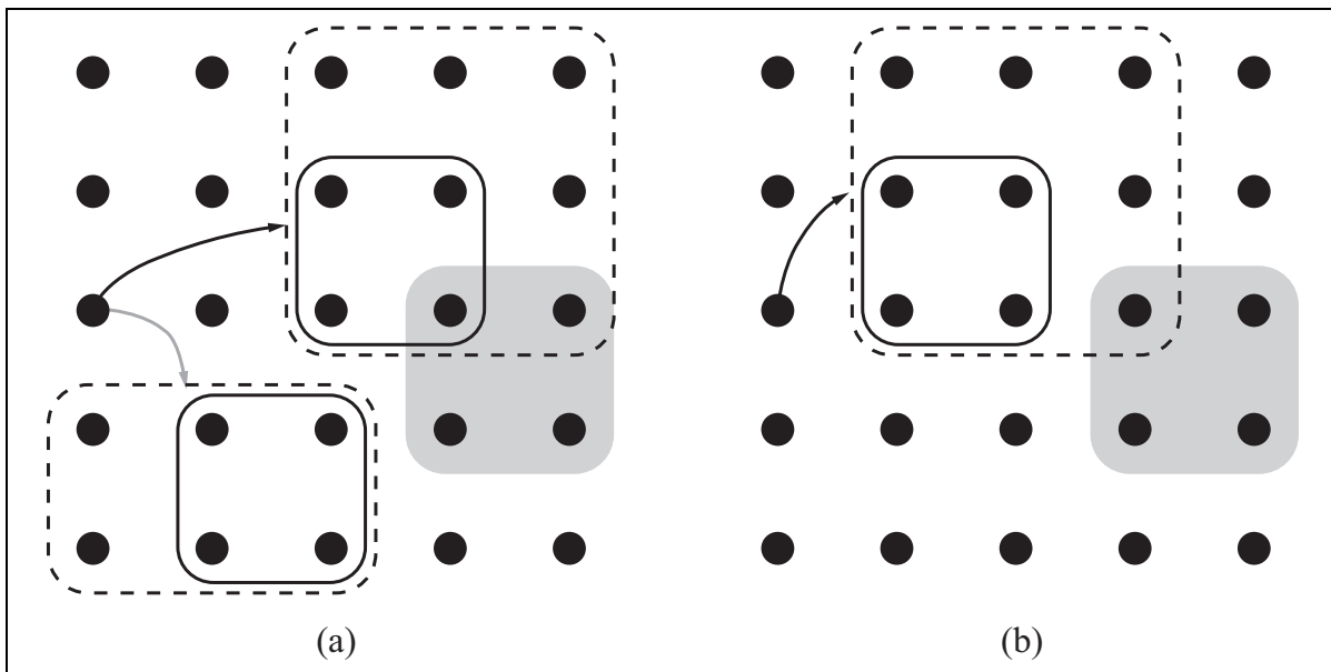
Figure 11.7 Goal achievement for high-level plans with approximate descriptions. The set of goal states is shaded. For each plan, the pessimistic (solid lines) and optimistic (dashed lines) reachable sets are shown. (a) The plan indicated by the black arrow definitely achieves the goal, while the plan indicated by the gray arrow definitely doesn't. (b) A plan that would need to be refined further to determine if it really does achieve the goal.
