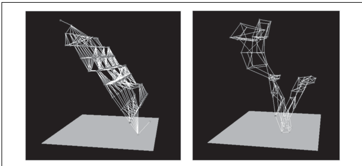
Figure 10.6 Two state spaces from planning problems with the ignore-delete-lists heuristic. The height above the bottom plane is the heuristic score of a state; states on the bottom plane are goals. There are no local minima, so search for the goal is straightforward. From Hoffmann (2005).
