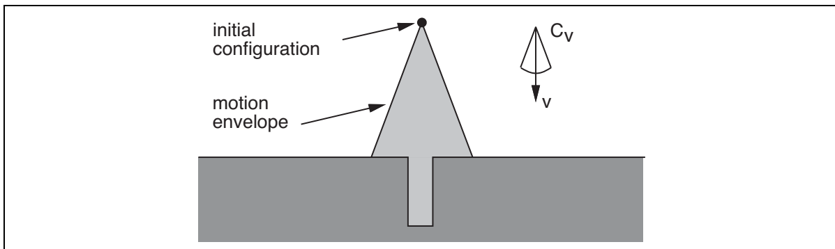
Figure 25.19 A two-dimensional environment, velocity uncertainty cone, and envelope of possible robot motions. The intended velocity is v , but with uncertainty the actual velocity could be anywhere in C_v , resulting in a final configuration somewhere in the motion envelope, which means we wouldn't know if we hit the hole or not.
